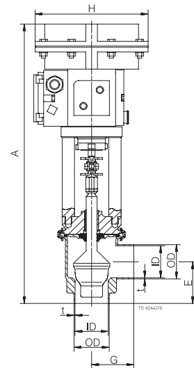
a. SPC-2, normally open (NO).
