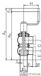
b. Change-over valve.
